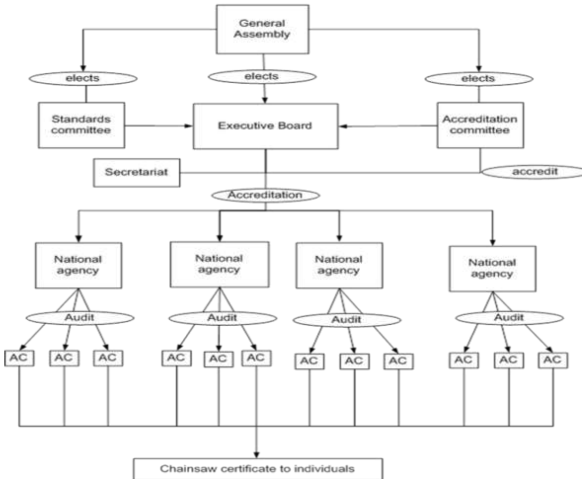
Organisational Chart
